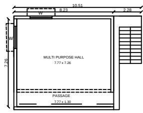
PROPOSED FIRST FLOOR PLAN
