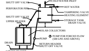
DETAILS OF SOLAR WATER HEATING SYSTEM
