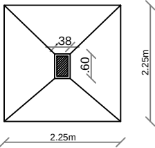
TYPICAL SECTION OF FOOTING
