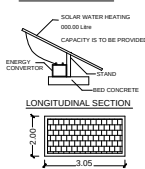
SOLAR SYSTEM
