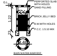
RAIN WATER HARVEST
