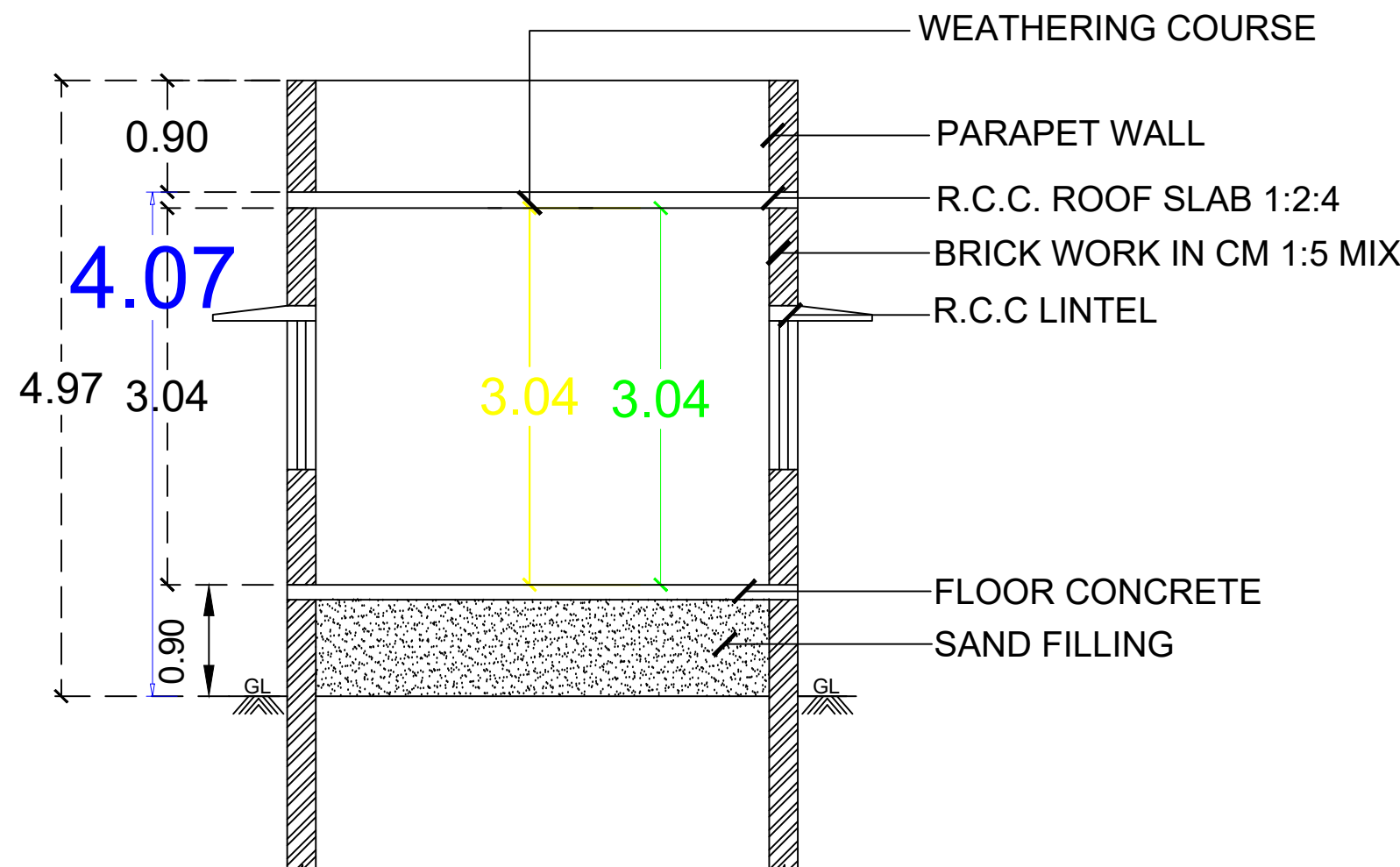
SECTION A1-A1
