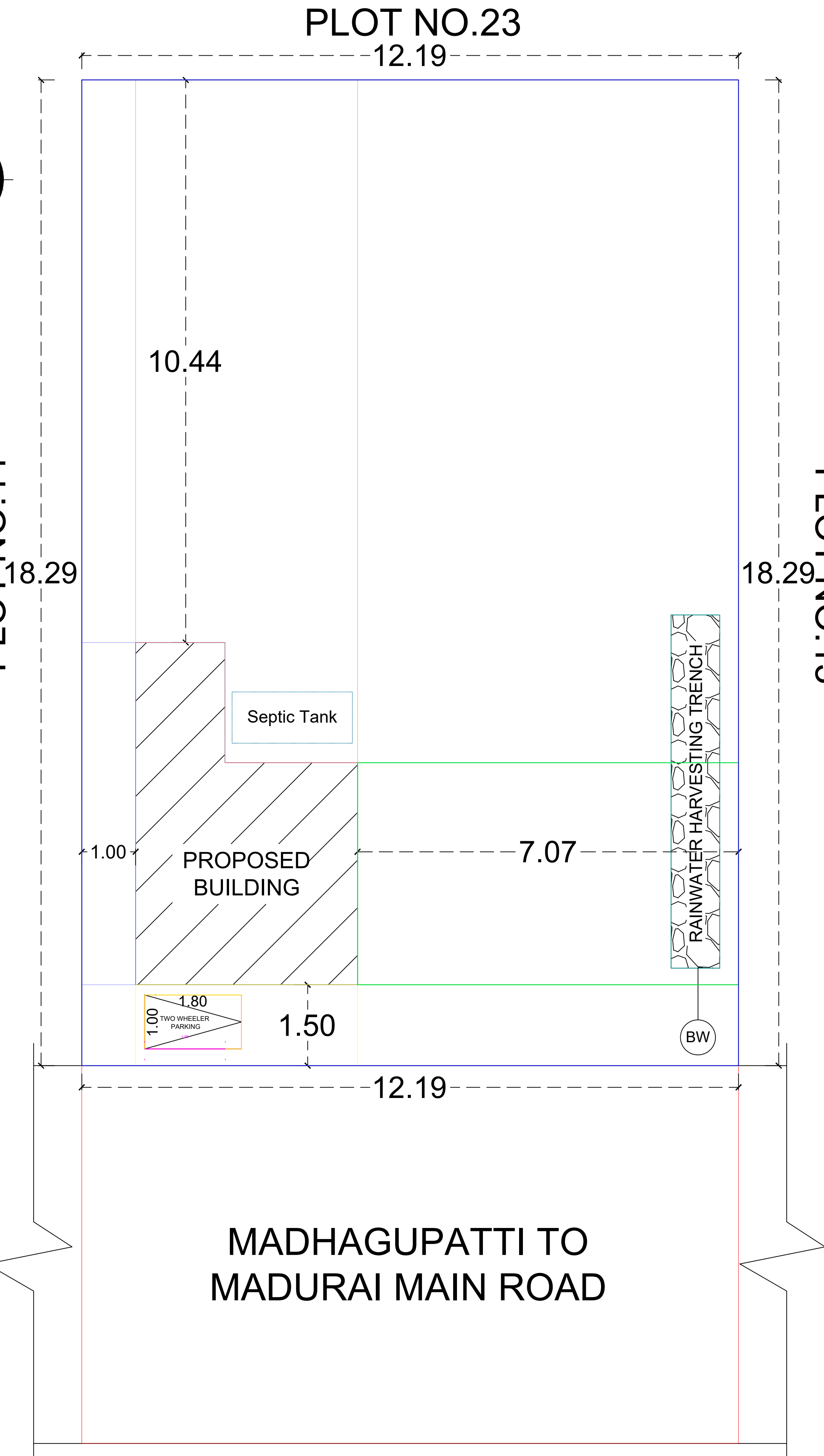
SITE PLAN (1:100)
