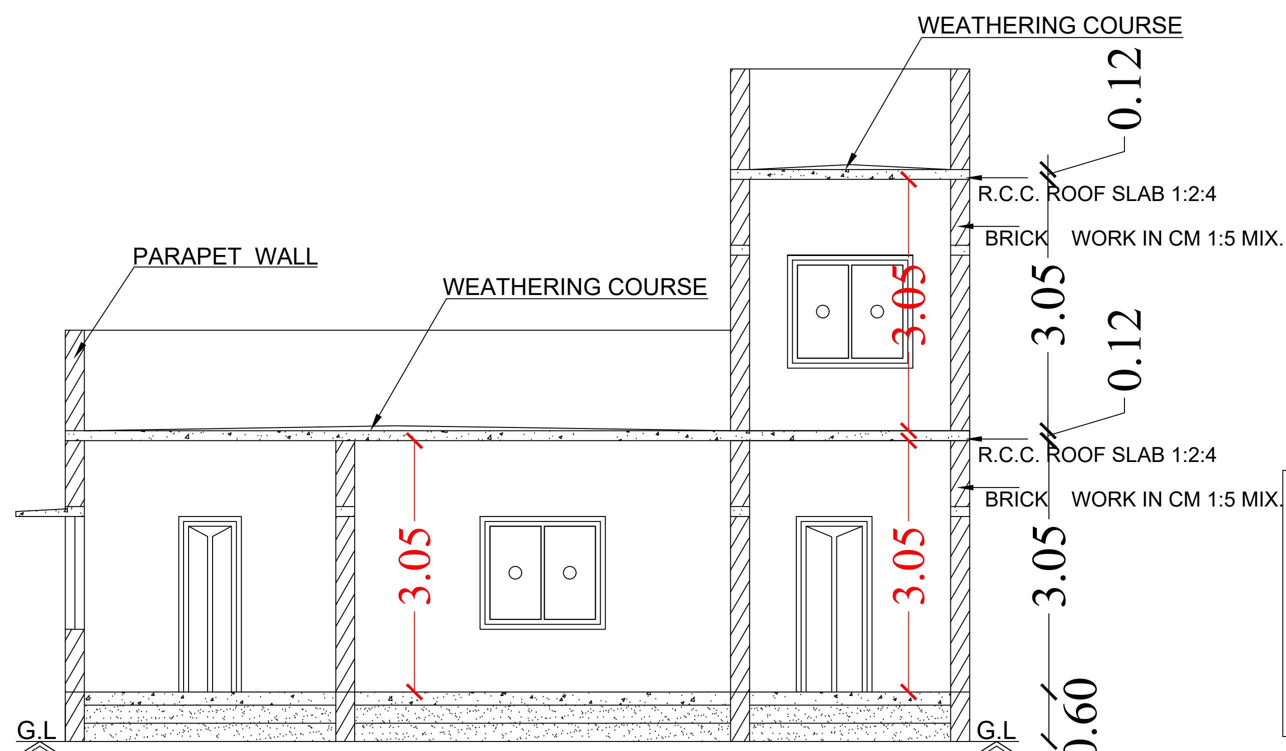
Section on-"AA"
