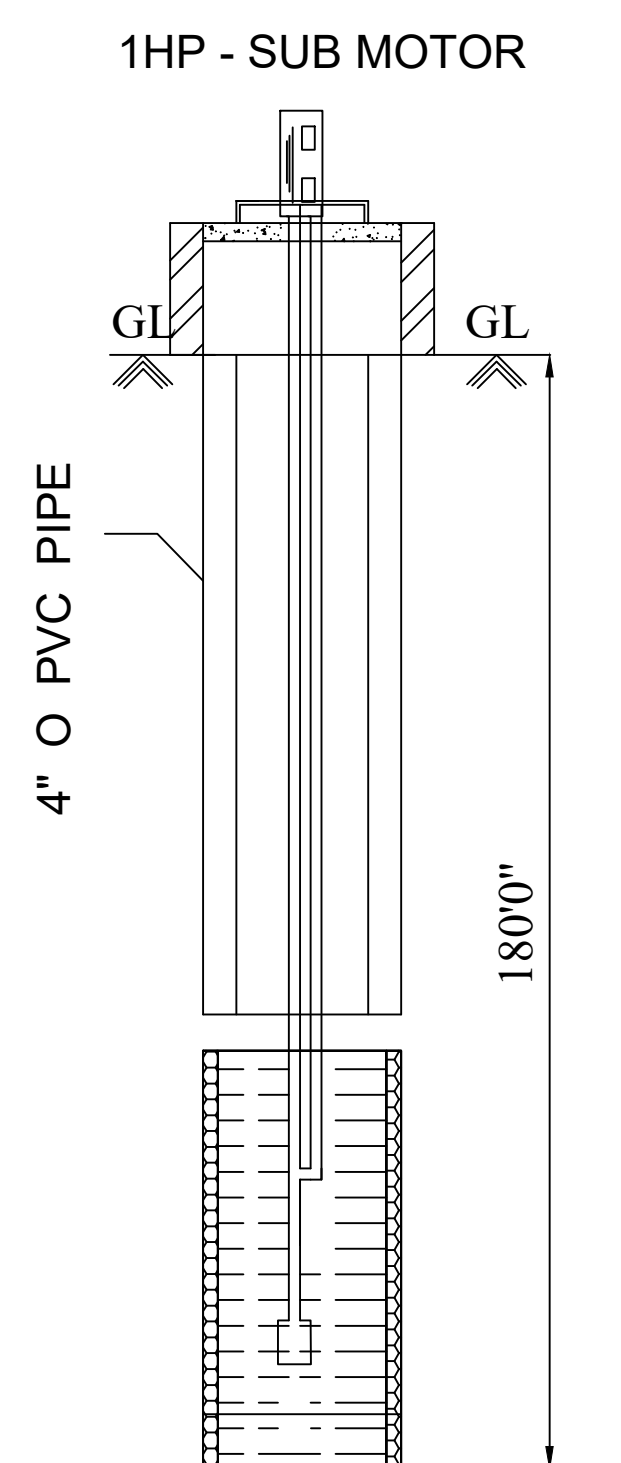
Bore Well Details
