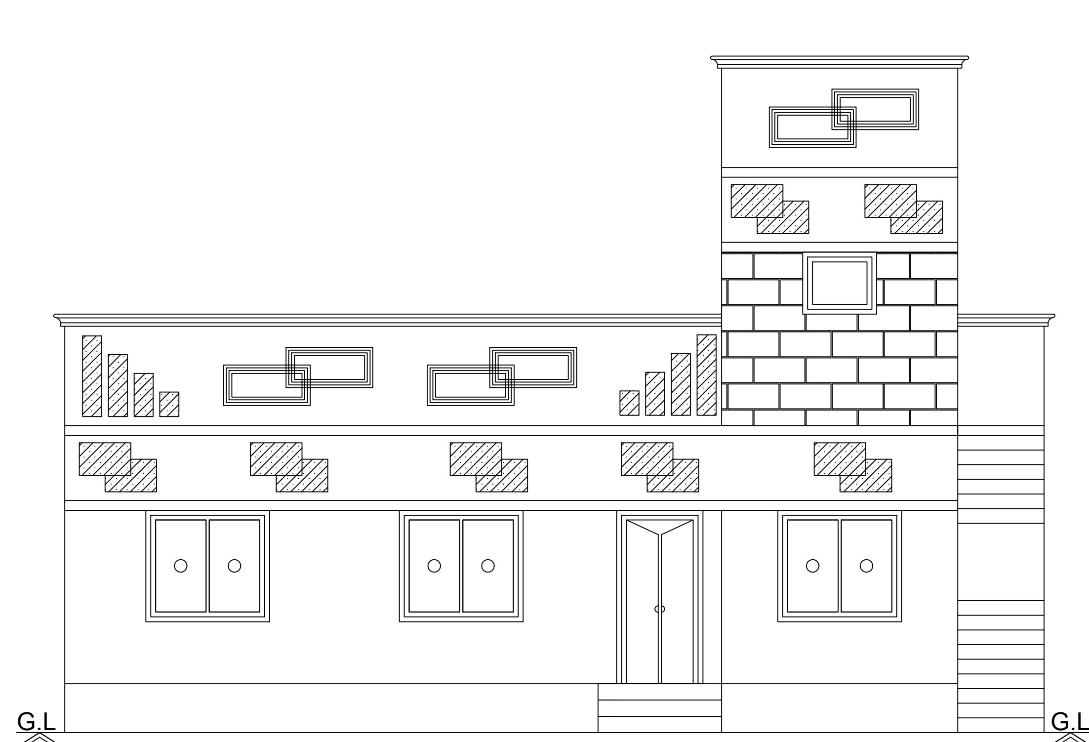
Front Elevation
