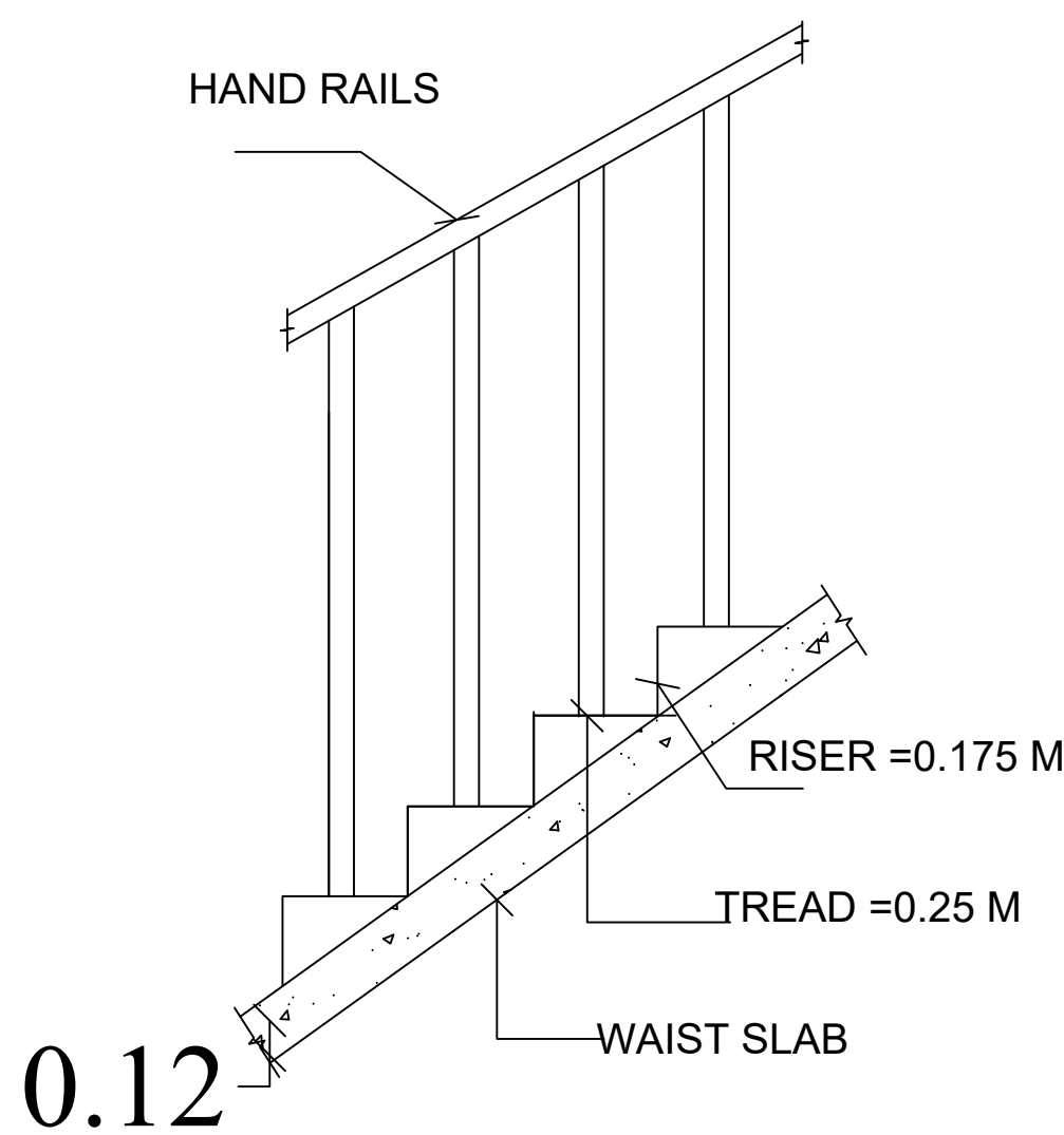
STAIR CASE DETAILS
