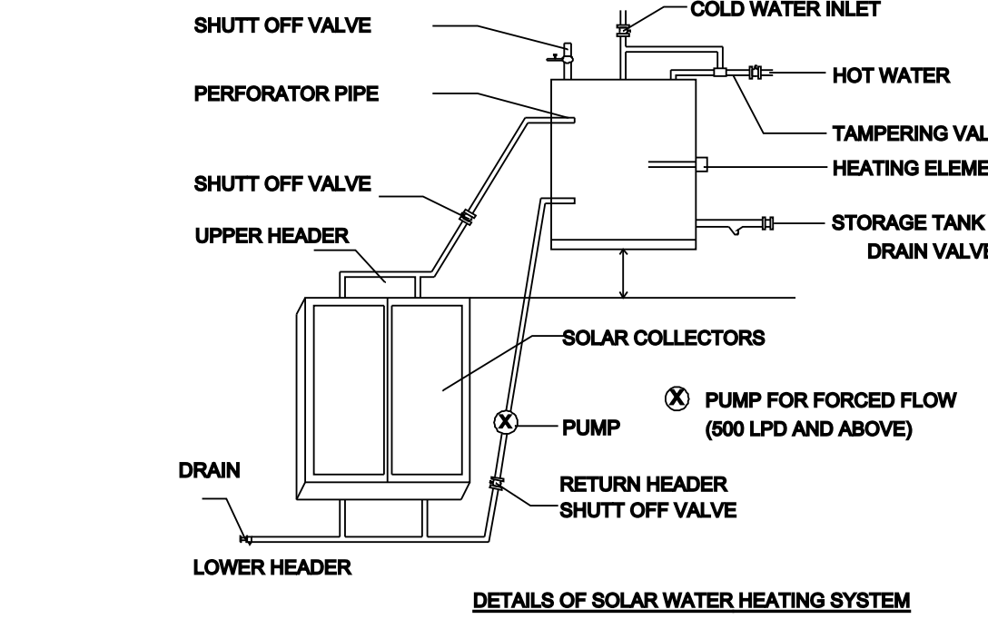
DETAILS OF SOLAR WATER HEATING SYSTEM
