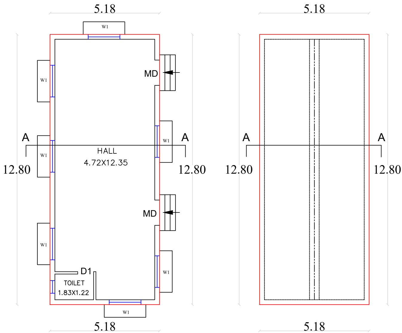
PROPOSED GROUND FLOOR PLAN TOP VIEW PLAN
