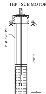
BOREWELL DETAILS
