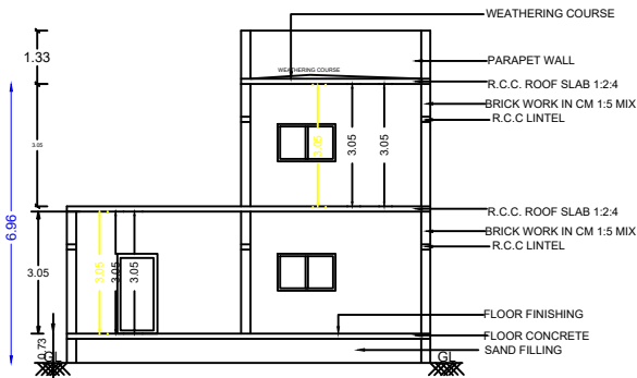
SECTION A1-A1
