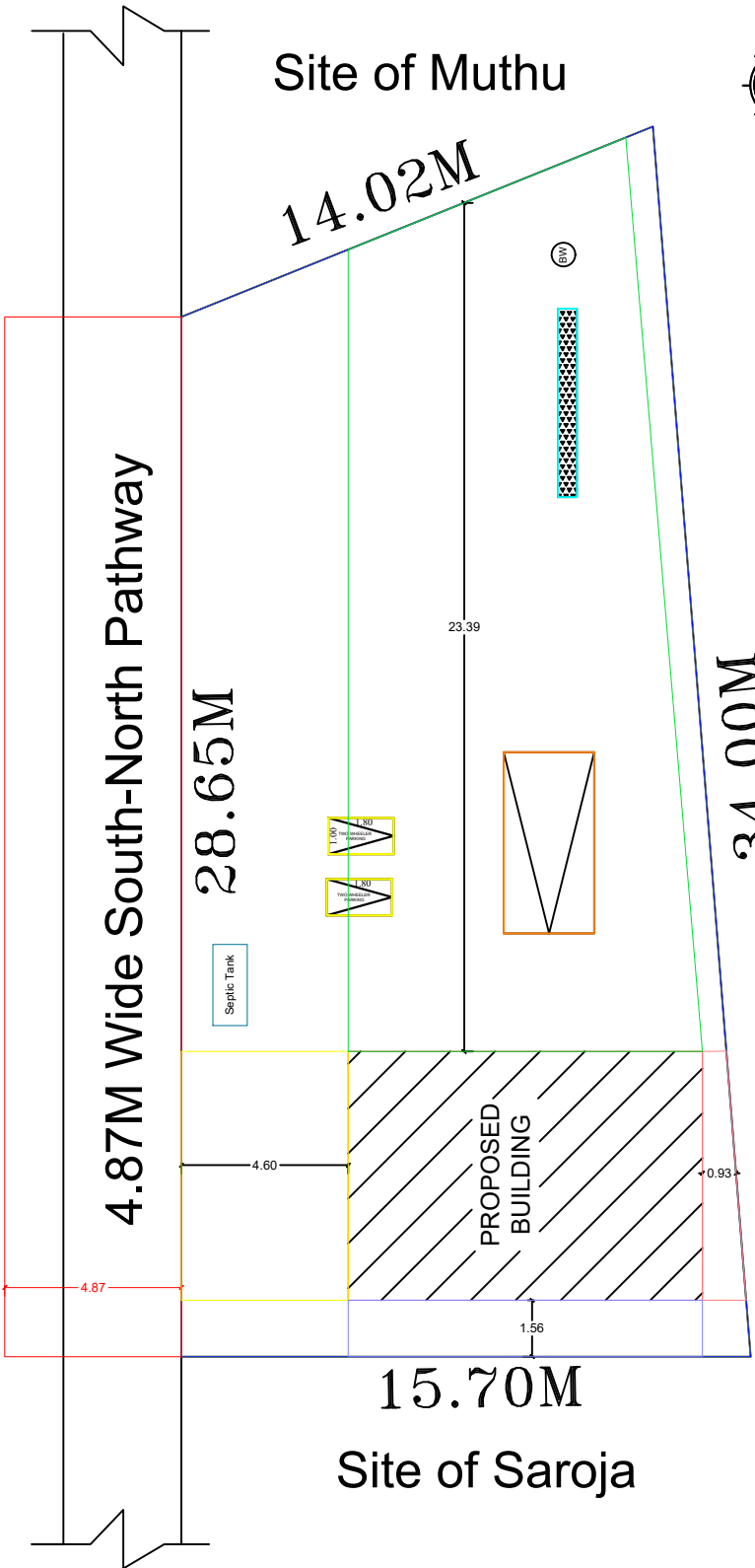
SITE PLAN
