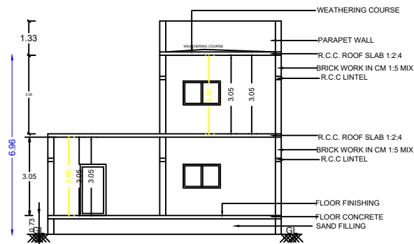
SECTION A1-A1
