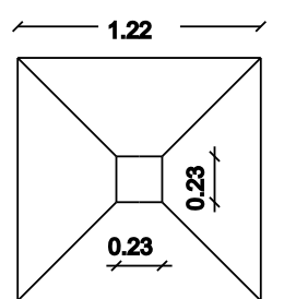
FOUNDATION DETAILS
