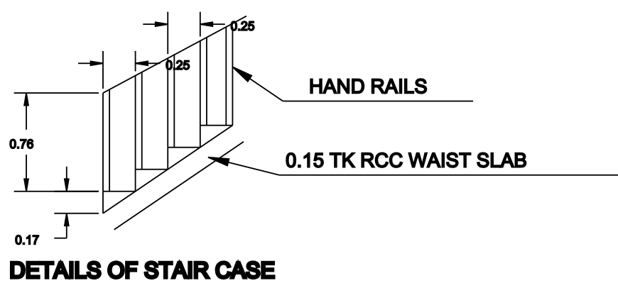
DETAILS OF STAIR CASE
