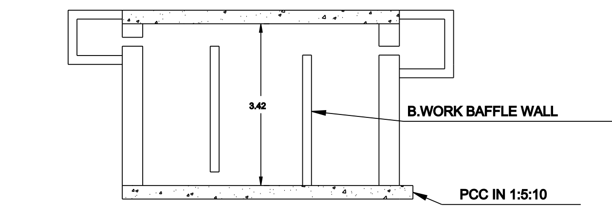
SECTION
