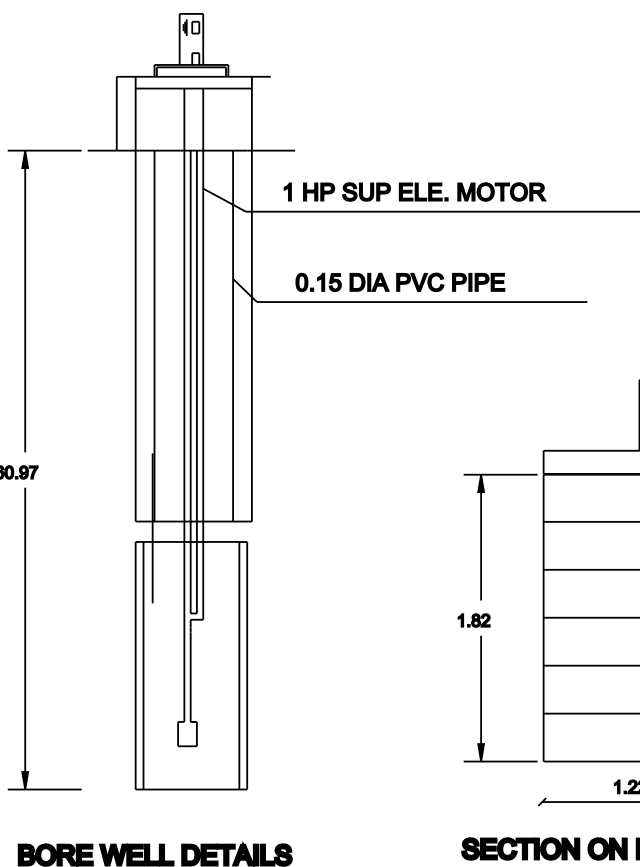
BORE WELL DETAILS
