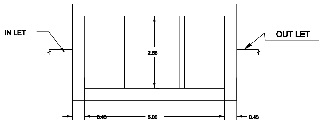
SEPTIC TANK DETAILS
