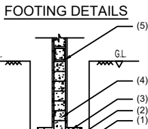
FOOTING DETAILS
