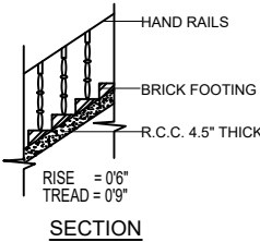
SEPTIC TANK DETAILS STAIR CASE DETAILS
