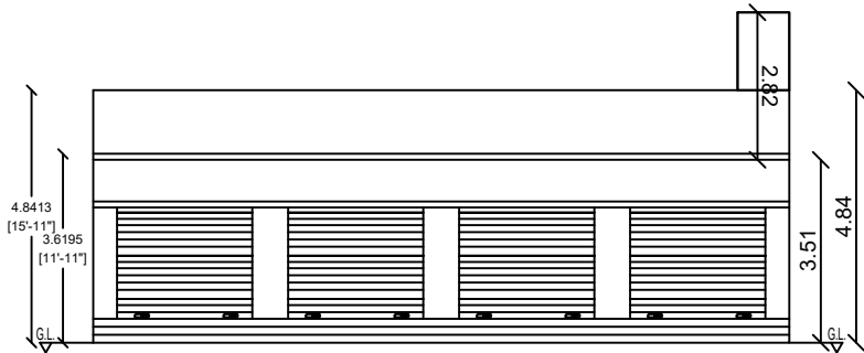
ELEVATION ON WEST
