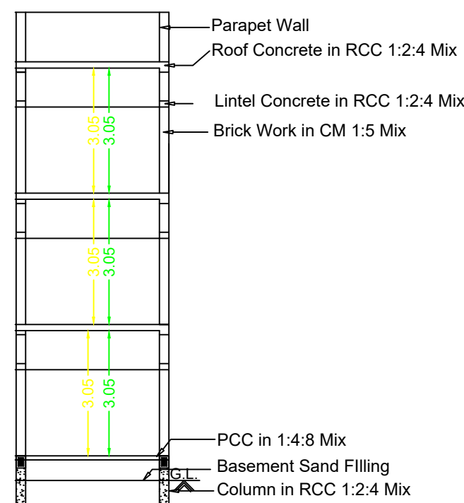
Section RR
