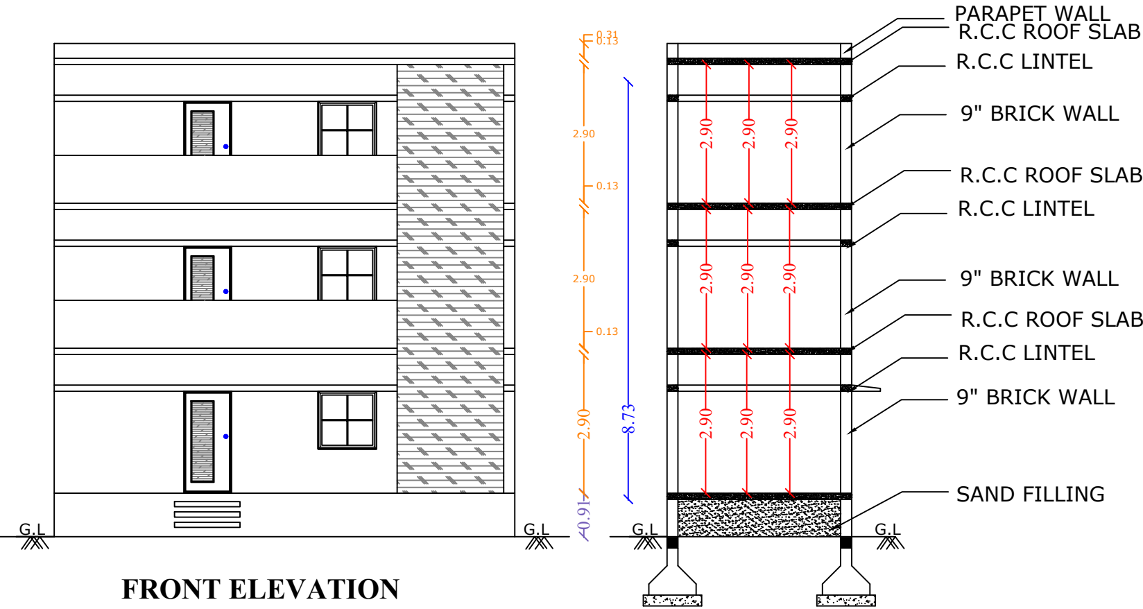
FRONT ELEVATION
