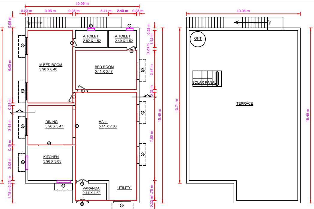
TERRACE PLAN
