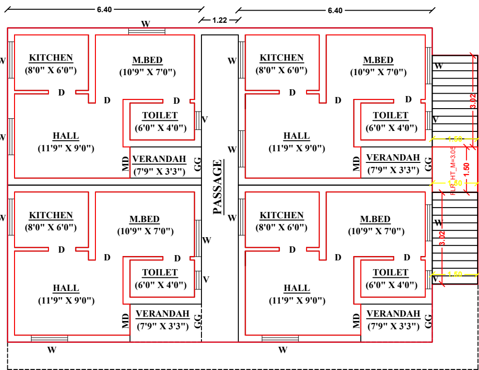
EXT GROUND FLOOR PLAN
