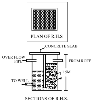
SECTIONS OF R.H.S.
