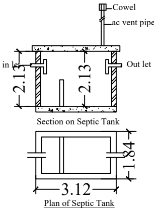
Plan of Septic Tank
