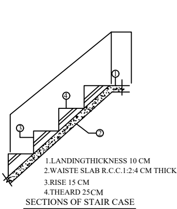
SECTIONS OF STAIR CASE
