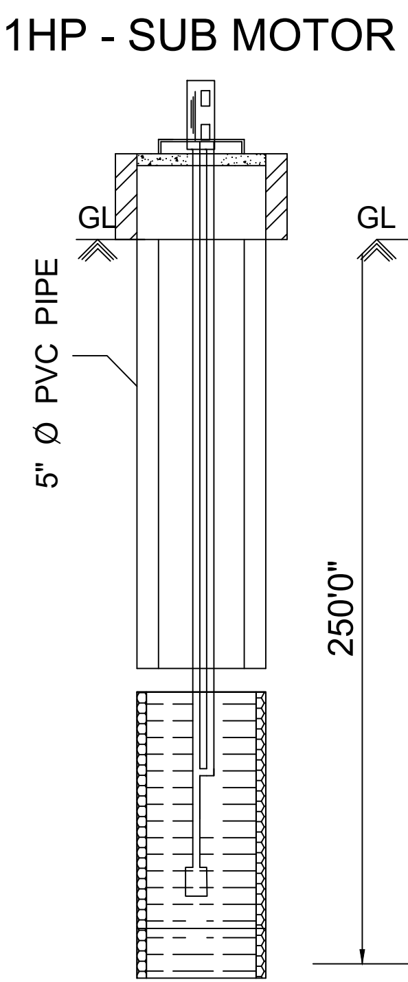
BOREWELL DETAILS
