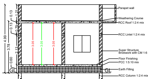
SECTION ON "VR"
