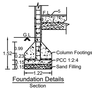
Foundation Details Section
