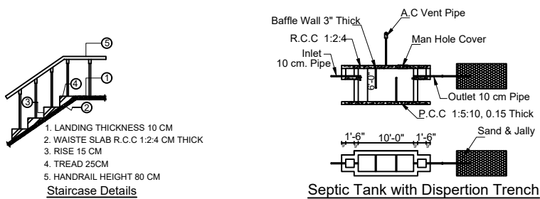
Septic Tank with Dispersion Trench
