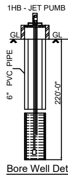
Bore Well Details
