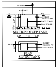
PLAN SEPTIC TANK
