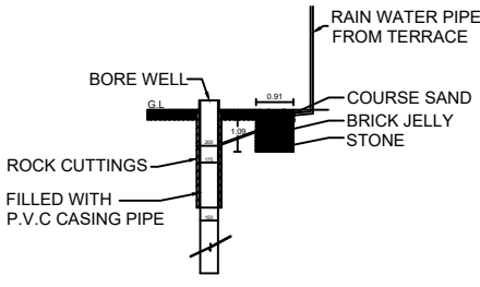
RAIN WATER HARVESTING DETAIL
