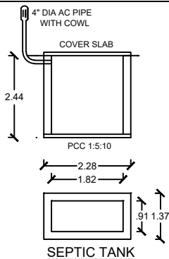
SEPTIC TANK
