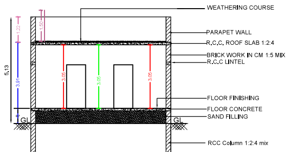
SECTION - 'RI'
