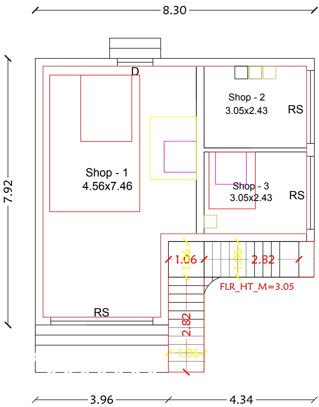
Ground Floor
