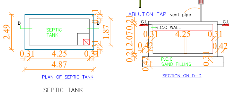
SEPTIC TANK
