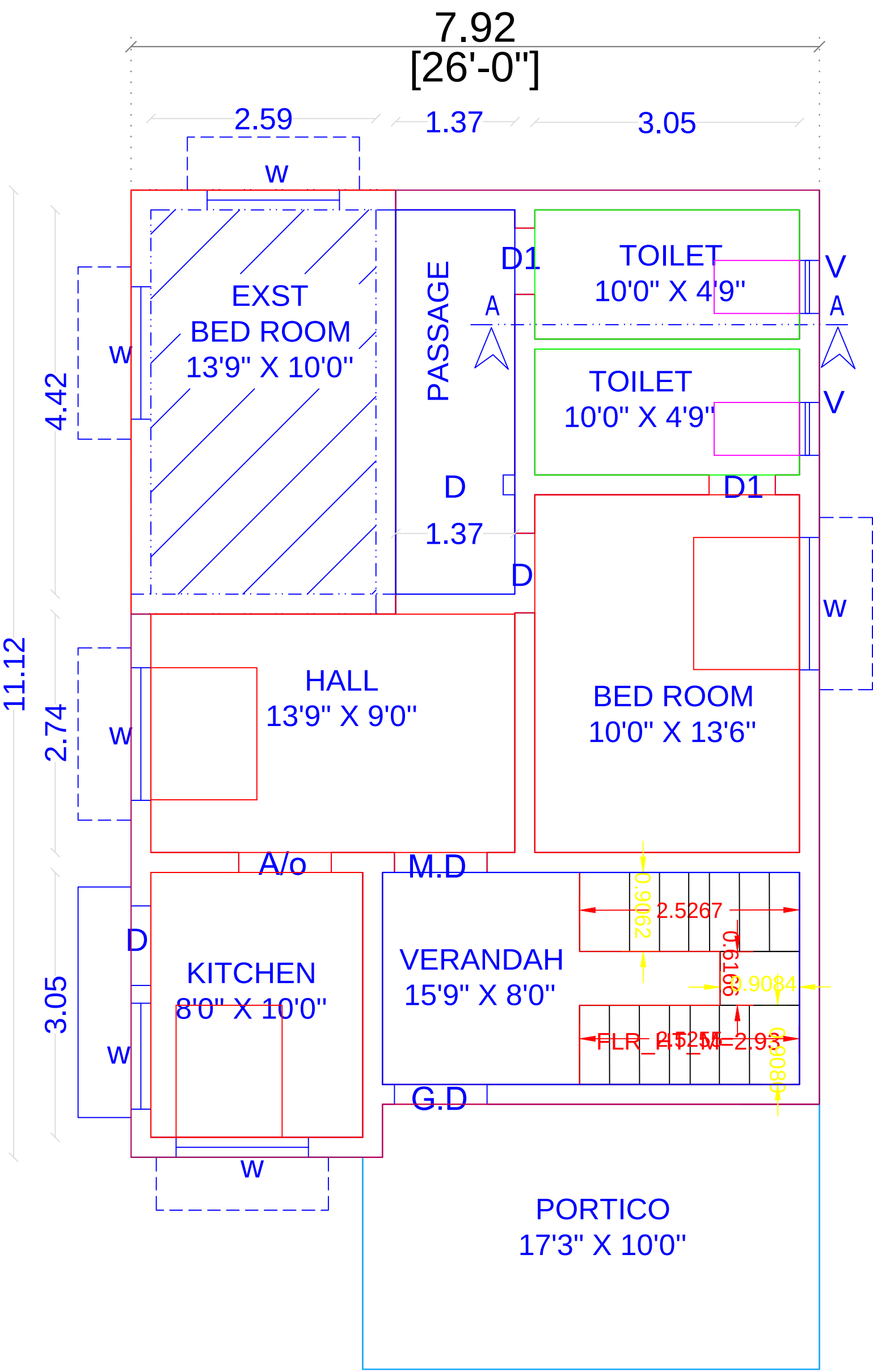
EXIST&PRO.GROUND FLOOR PLAN
