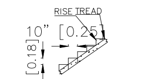
SECTION ON STAIRCASE (NOT TO SCALE)
