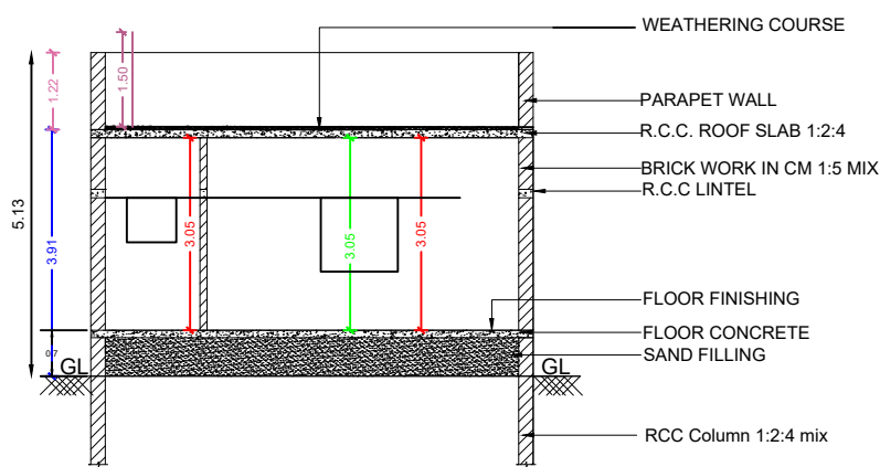
SECTION - 'RI'
