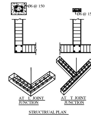
STRUCTURAL PLAN
