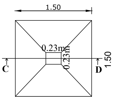
SECTION - 'CD' FLOORING CONCRETE
