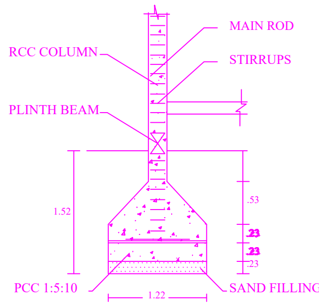
COLUMN DETAILS
