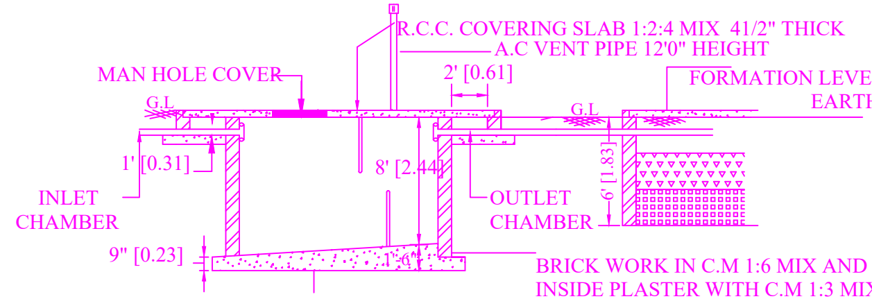
SEPTIC TANK
