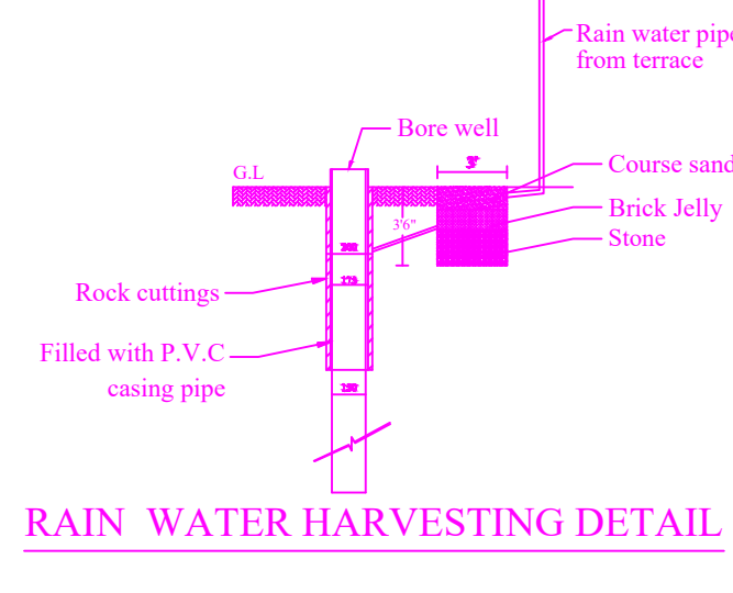
RAIN WATER HARVESTING DETAIL
