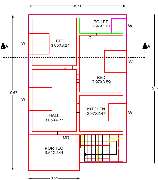
EXISTING RESIDENTIAL GROUND FLOOR BUILDING
