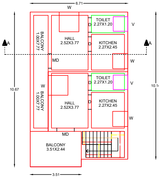
PROPOSED RESIDENTIAL GROUND FLOOR PLAN
