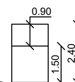
RAIN WATER HARVESTING TRENCH RW.H. CAPACITY: L=2000 SUMP SUMP_CAPACITY: L=2000
