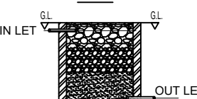
RAINWATER STORAGE PIT DETAILS
