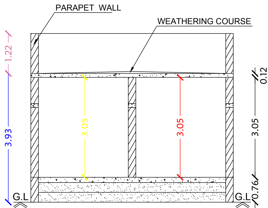
Section on-"AA"
