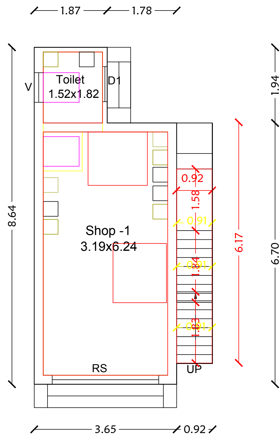
Ground Floor
