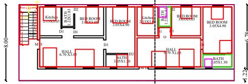
F. FLOOR PLAN
