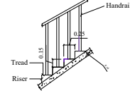
STAIRCASE DETAIL
