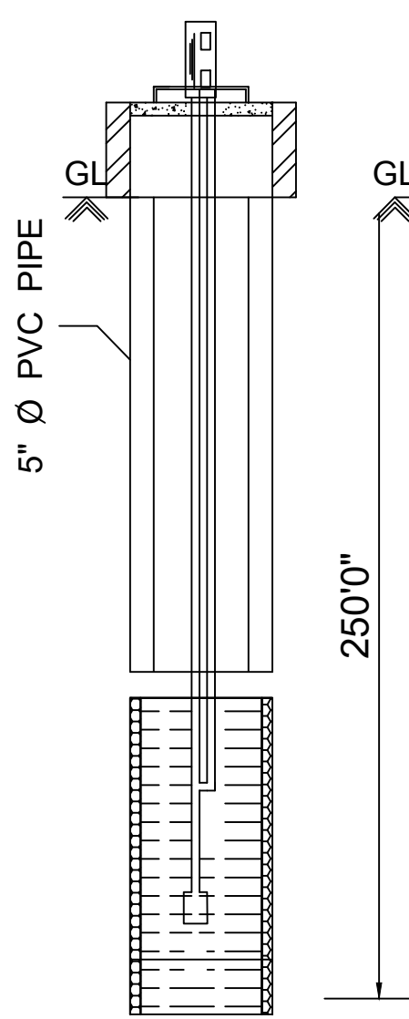
BOREWELL DETAILS
