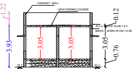
Section on-"AA"
