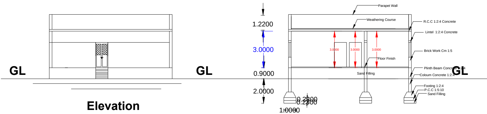
Section - AA
