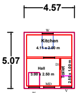
GROUND FLOOR EAST FACING
