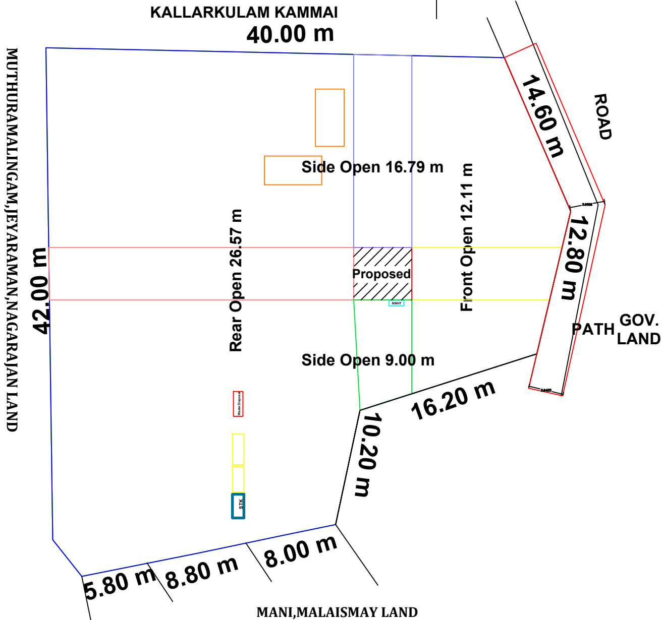
Site Plan
