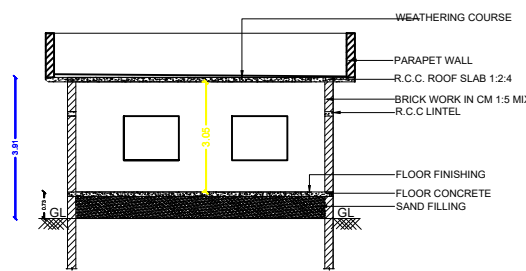
SECTION ON "R-I"
