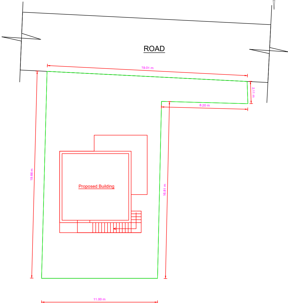
SITE PLAN
