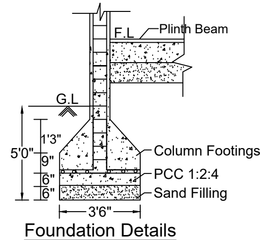
Foundation Details
