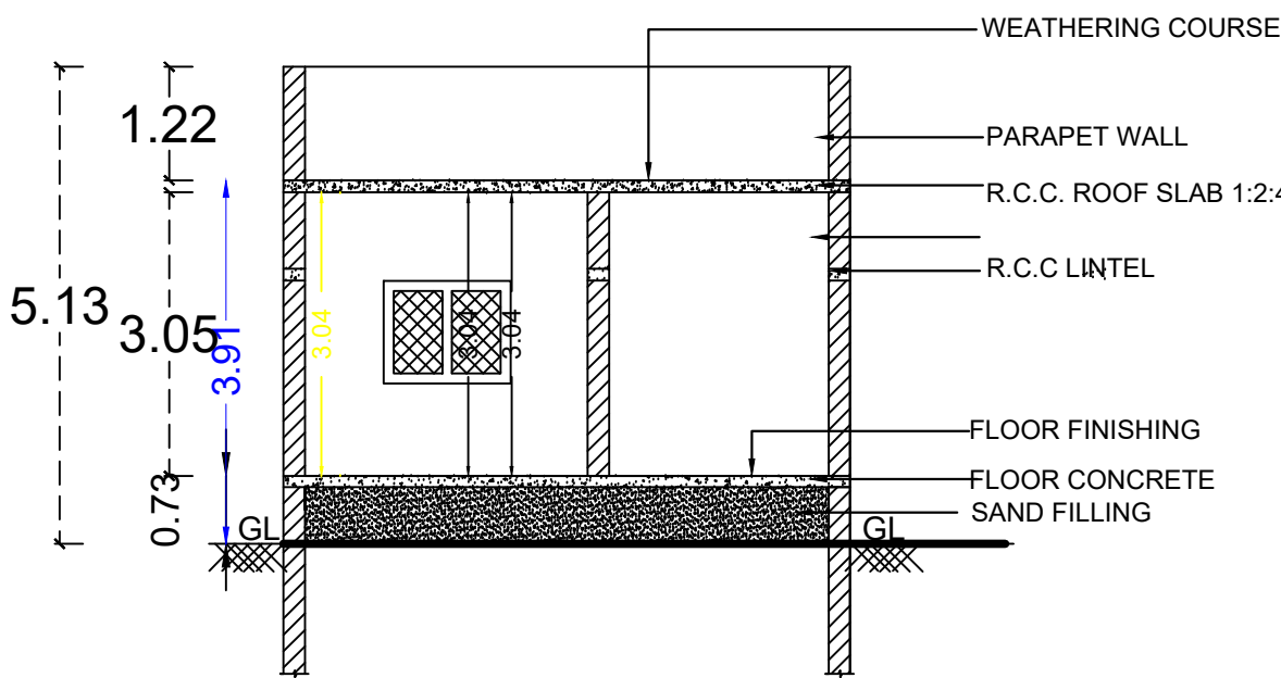
SECTION A1-A1
