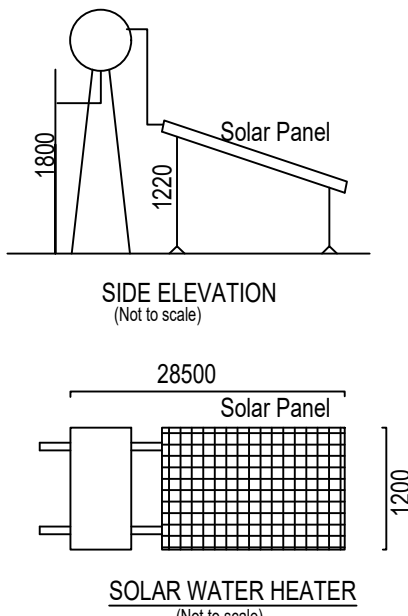
Solar Water Heater
