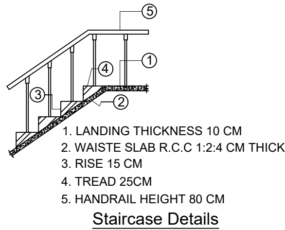
Staircase Details
