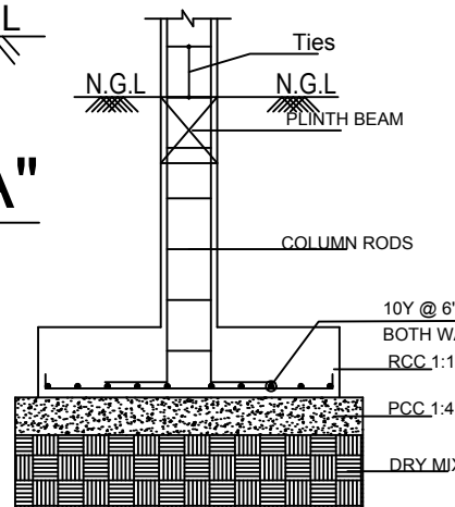
FOUNDATION DETAILS (Concentric Footing)
