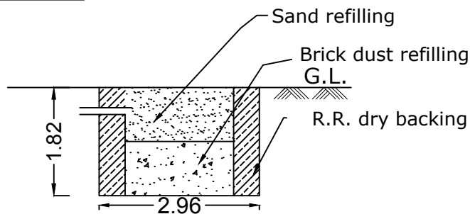
DETAILS OF RAIN WATER HARVESTING
