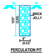
PERCOLATION PIT
