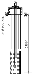
BOREWELL DETAILS
