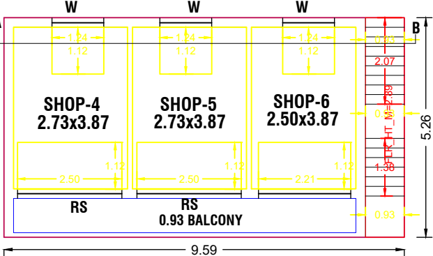
PRO.,FIRST FLOOR PLAN
