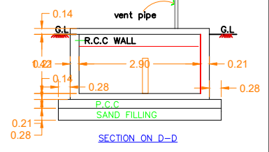
SCALE 1"=2'0"
