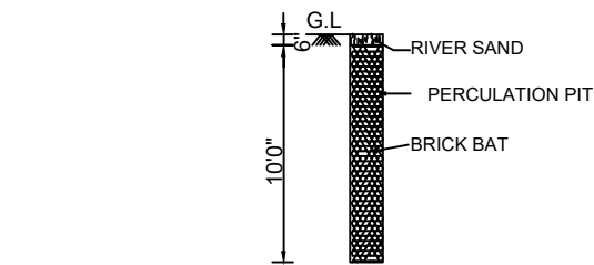
PERCULATION PIT
