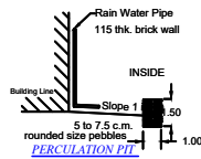
RAIN WATER PIPE
