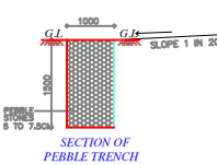
SECTION OF PEBBLE TRENCH
