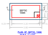
PLAN OF SEPTIC TANK
