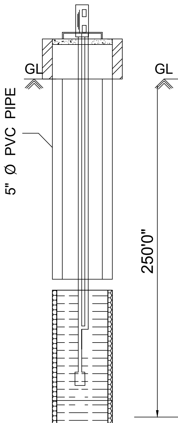
BOREWELL DETAILS
