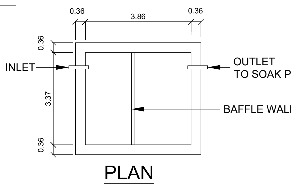
SEPTIC. TANK
