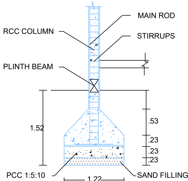
COLUMN DETAILS
