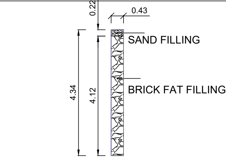
DETAILS OF PERCOLATION PIT
