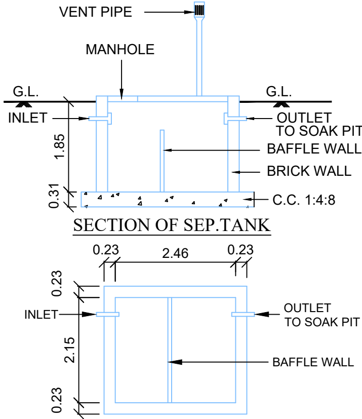
PLAN SEPTIC. TANK
