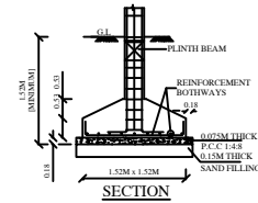
FOUNDATION DETAILS
