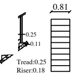
STAIRCASE DETAIL
