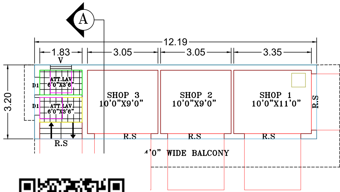
ROUND FLOOR PLAN
