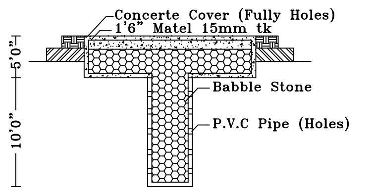
RAIN WATER STOREAGE TANK
