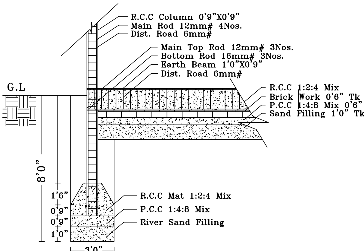
FOUNDATION DETAILS
