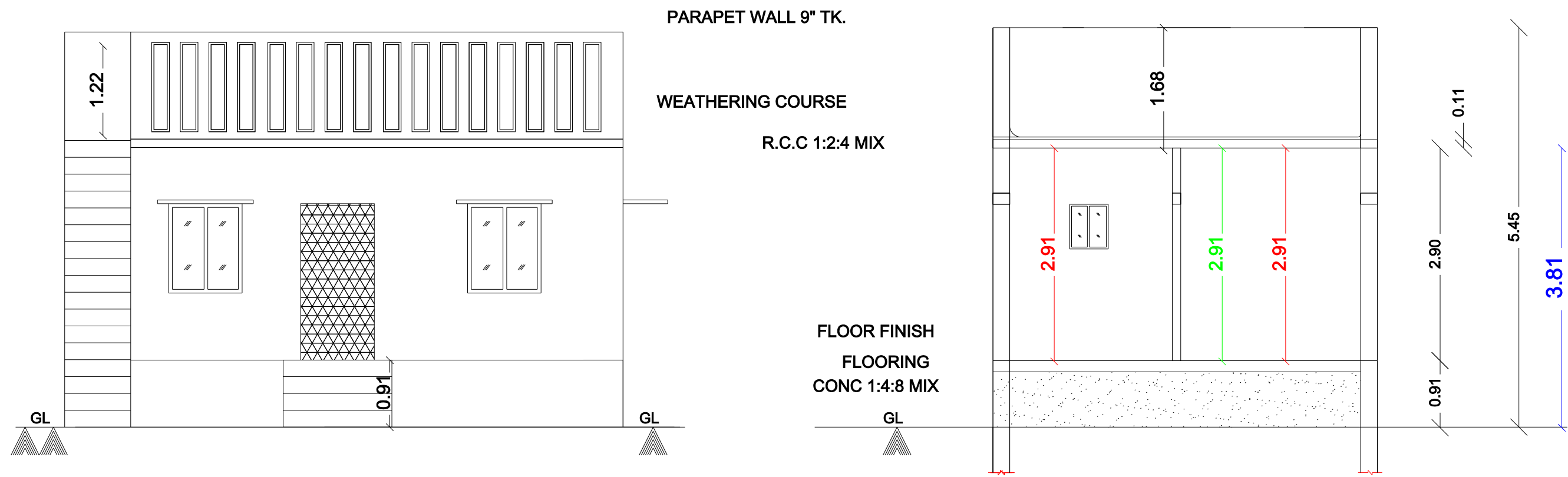
FRONT ELEVATION
