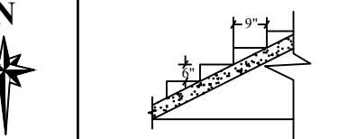
Staircase Detail Not To Scale
