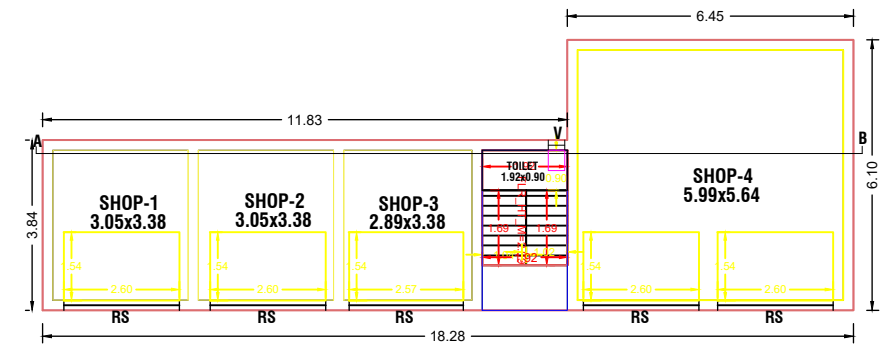
PRO.,GROUND FLOOR PLAN
