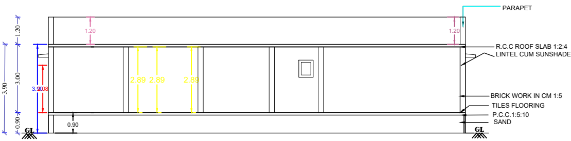
SECTION ON A-B
